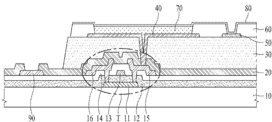
FIG. 1 (RELATED ART)
